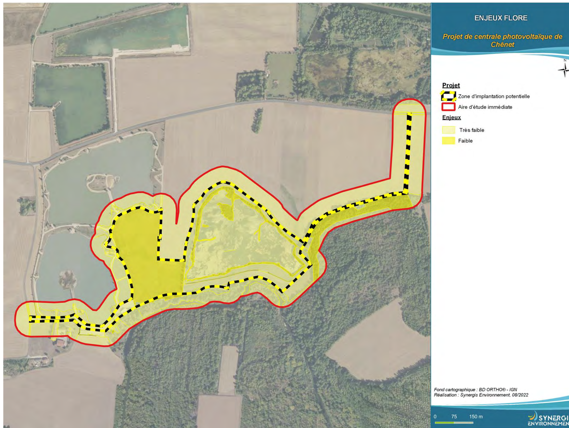
Figure 75 : Enjeux Flore
